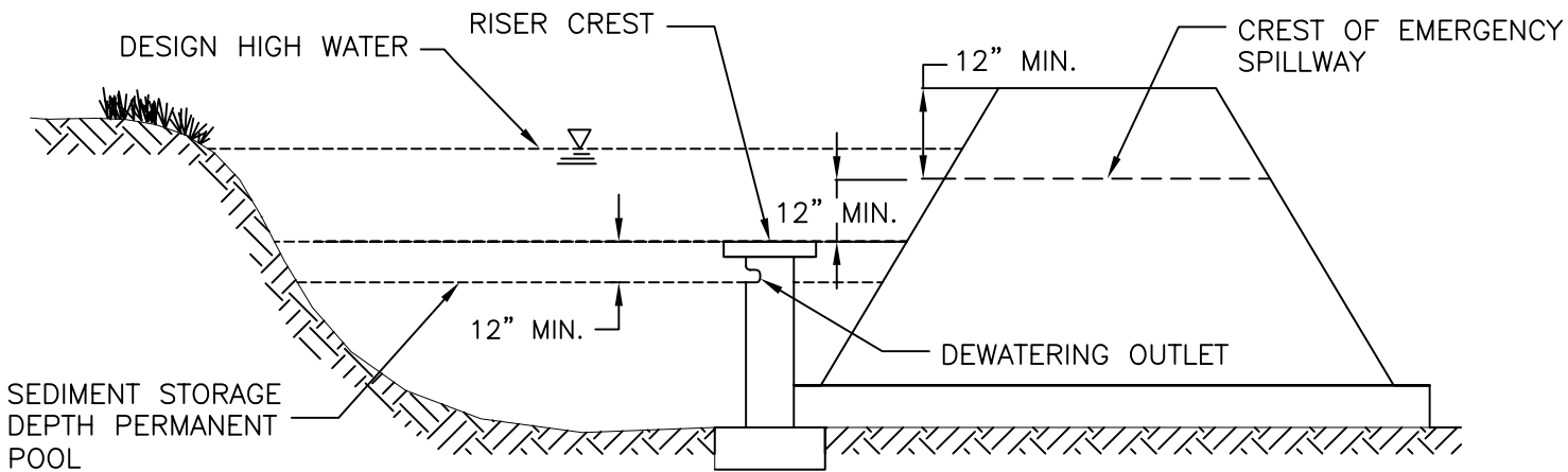
SIDE VIEW
