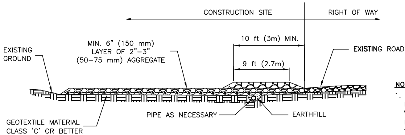
CONSTRUCTION ENTRANCE/EXIT SECTION VIEW A-A
