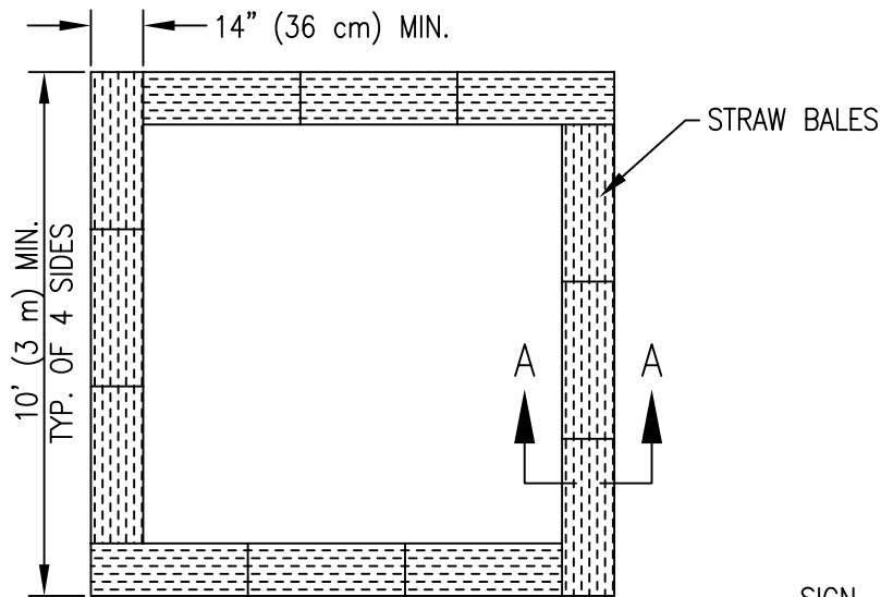
BALE CONFIGURATION
