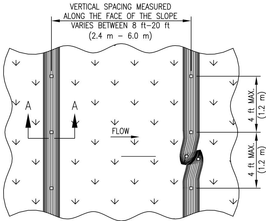
TYPICAL FIBER ROLL INSTALLATION
