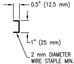
STAPLE DETAIL
