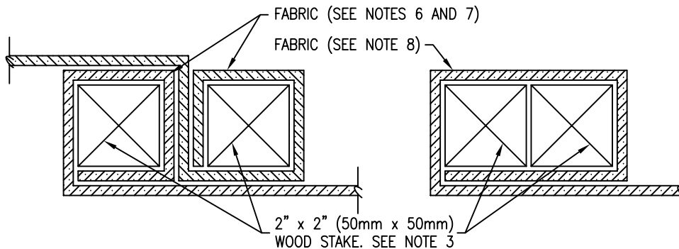
JOINT DETAIL
