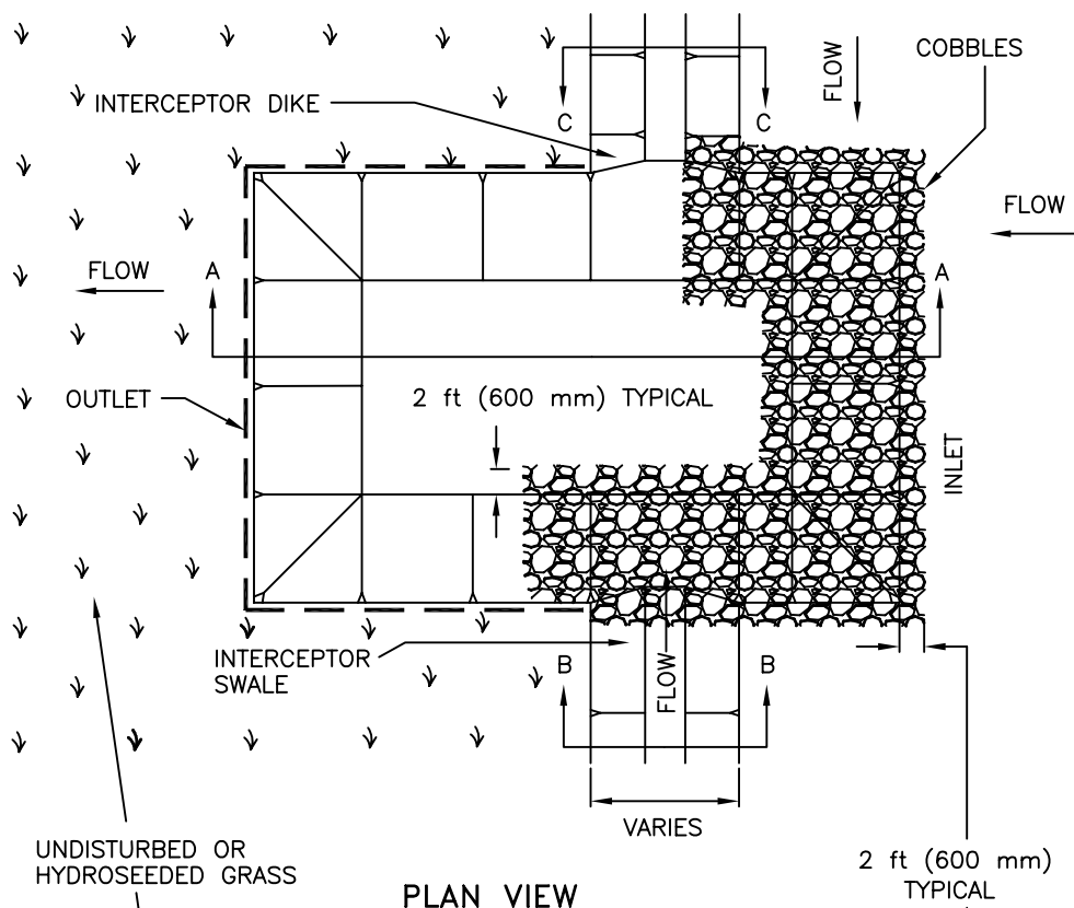
PLAN VIEW
