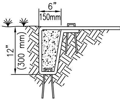
TERMINAL SLOPE AND CHANNEL ANCHOR TRENCH
