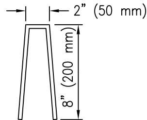
WIRE STAPLES
