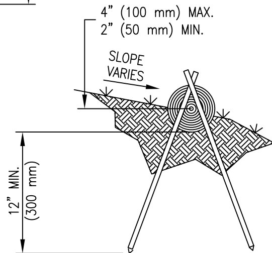
ALTERNATE STAKING DETAIL
