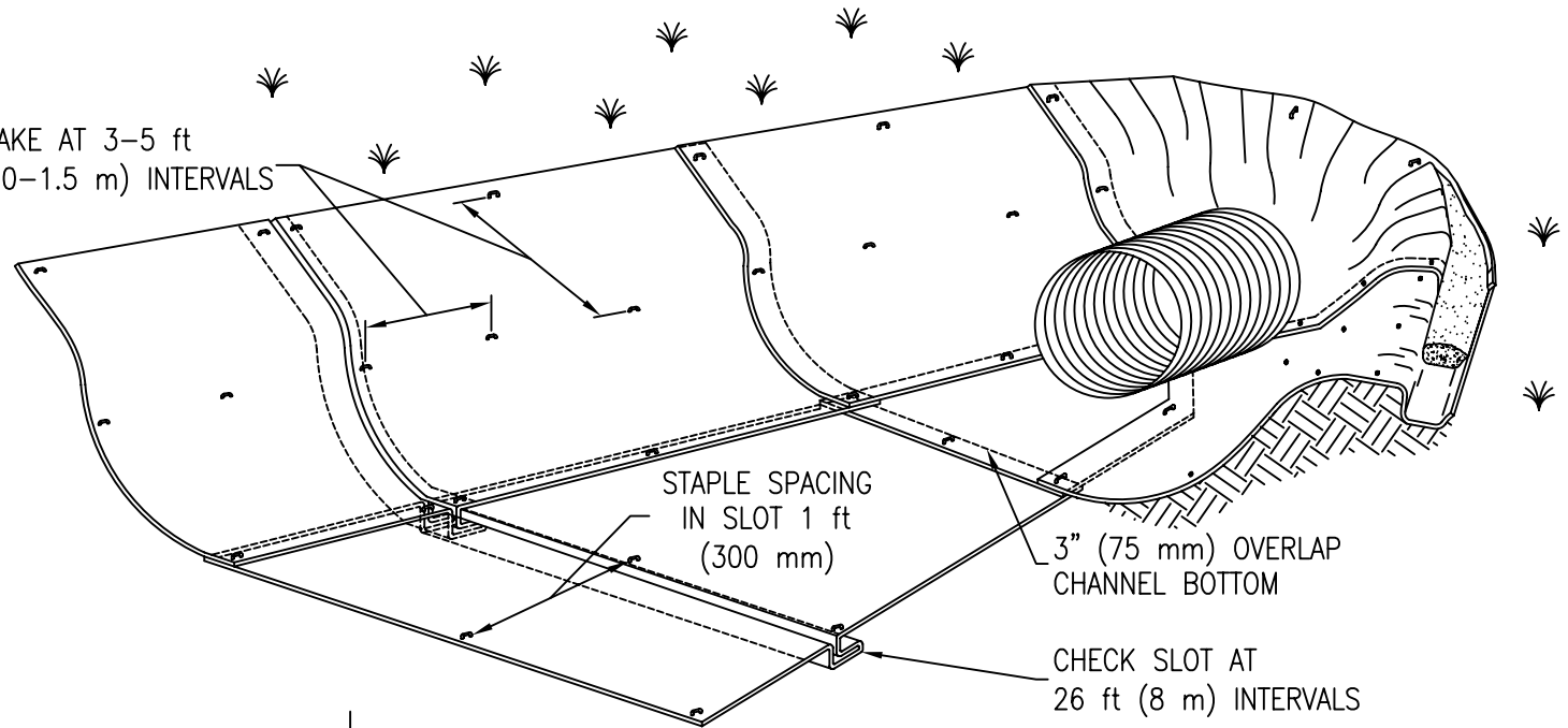
TYPICAL CHANNEL SOIL STABILIZATION
