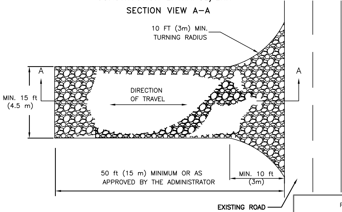
CONSTRUCTION ENTRANCE/EXIT PLAN VIEW
