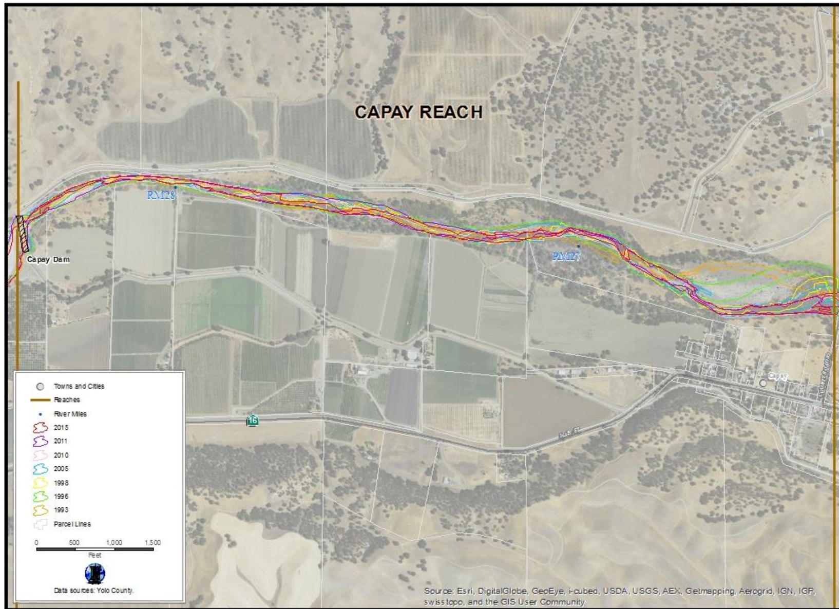
FIGURE 1.5: ACTIVE CHANNEL LOCATIONS IN THE CAPAY REACH IN 1996, 1998, 2005, 2006, 2011, AND 2015.
