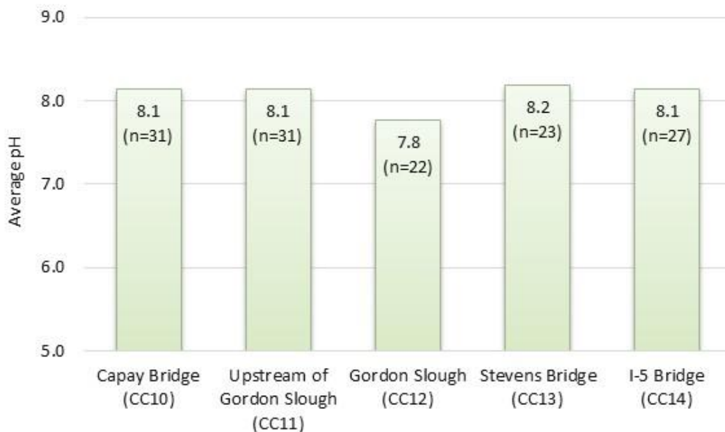
FIGURE 2.16: CACHE CREEK AVERAGE PH BY SAMPLE LOCATION.
