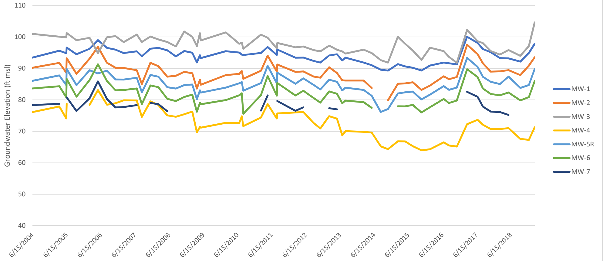
Chart 1 Water Levels 2004-19
