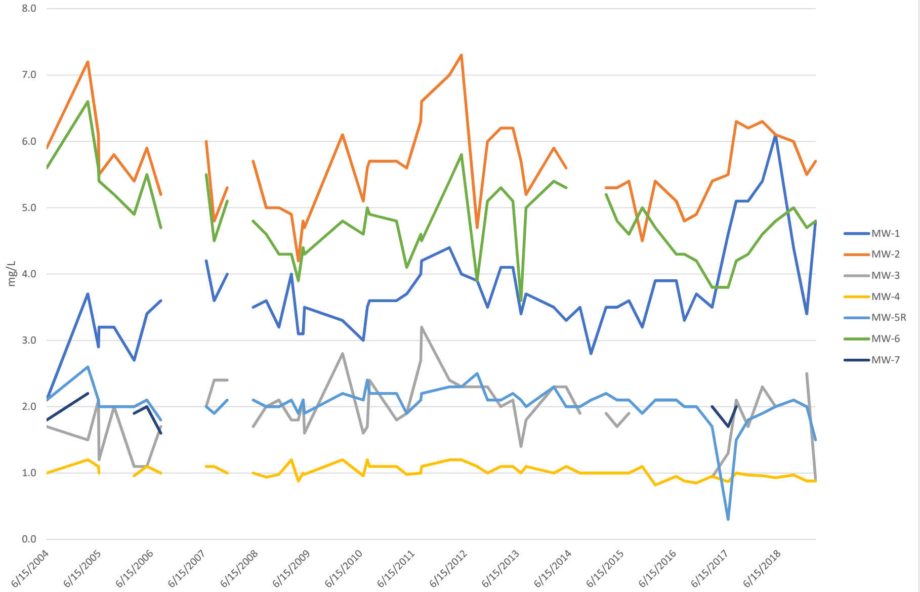
Chart 6 B Trends 2004-19
