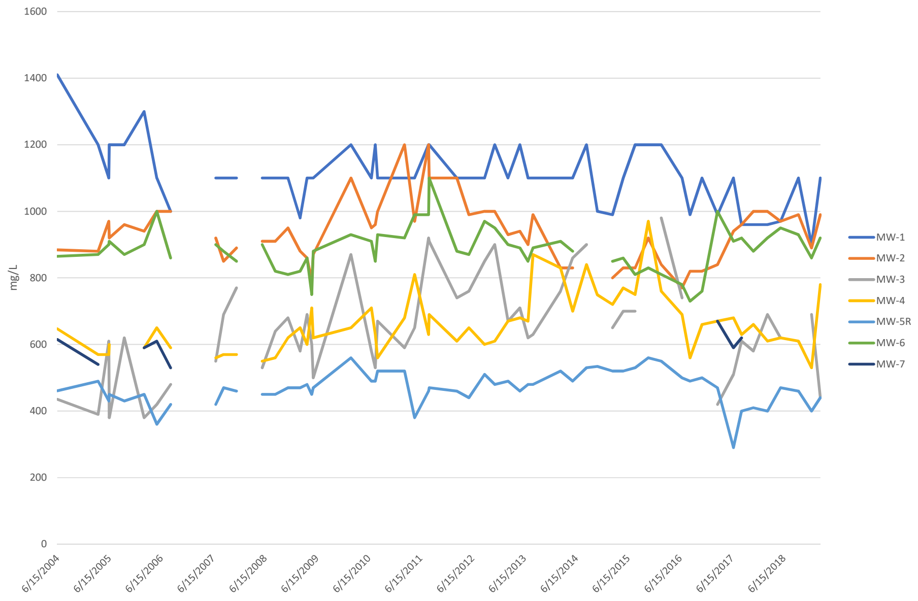
Chart 3 TDS Trends 2004-19
