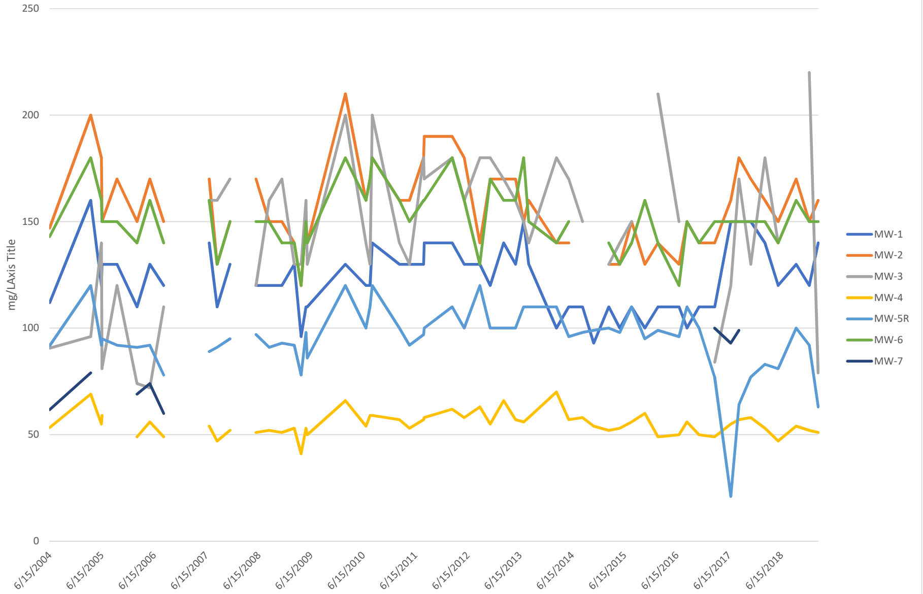
Chart 4 Na Trends 2004-19
