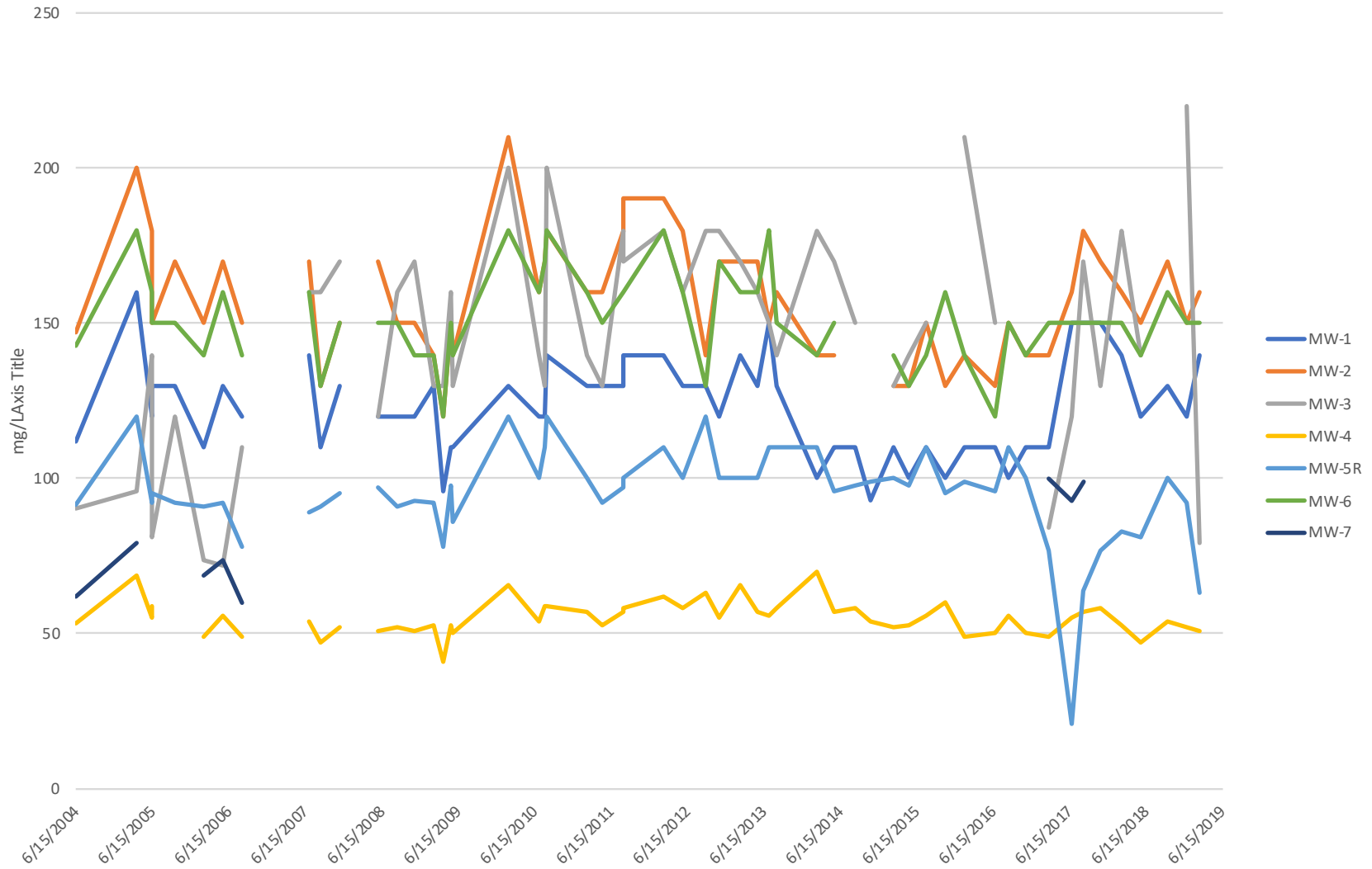
Chart 4 Na Trends 2004-19
