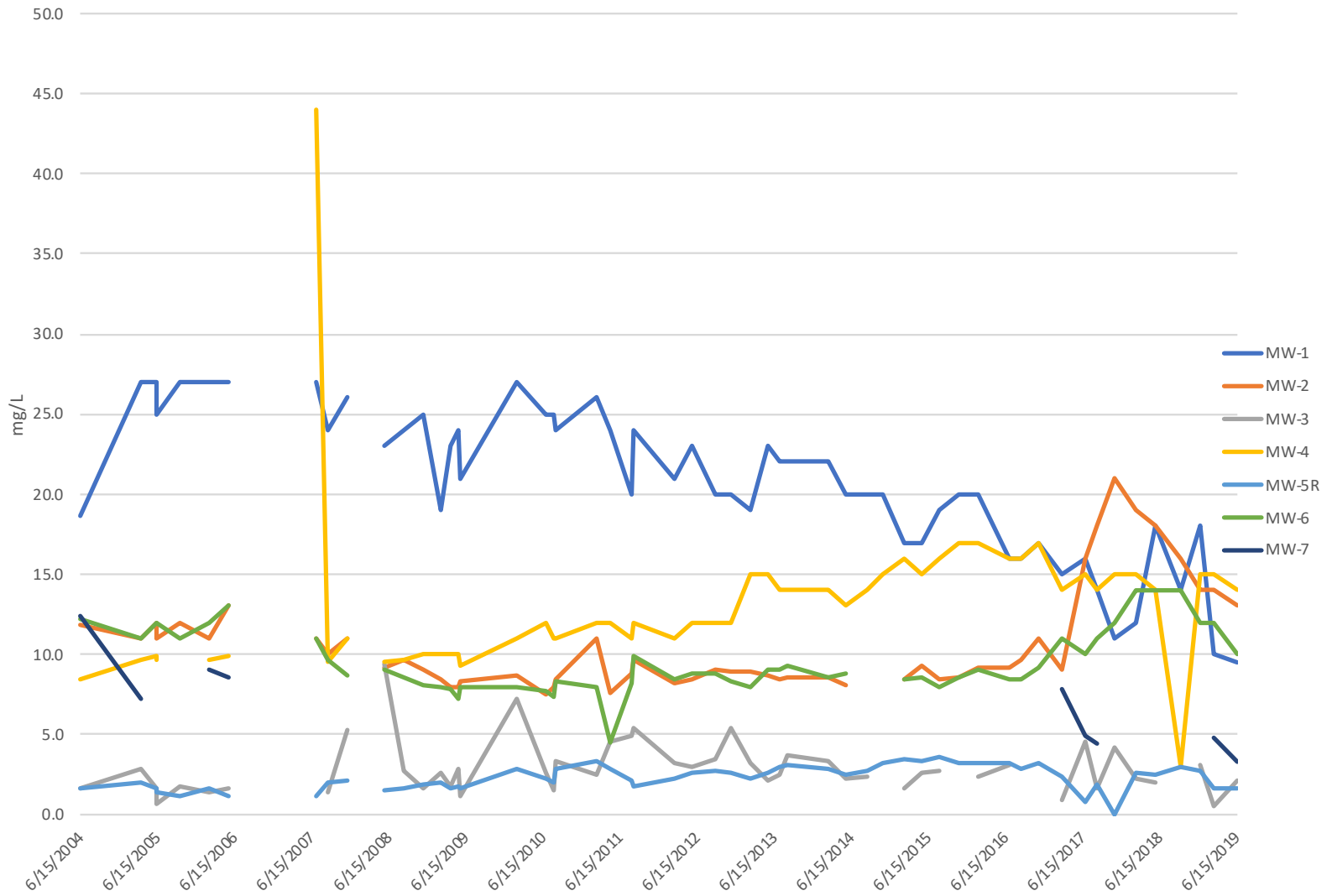
Chart 8 Total Nitrogen Trends 2004-19
