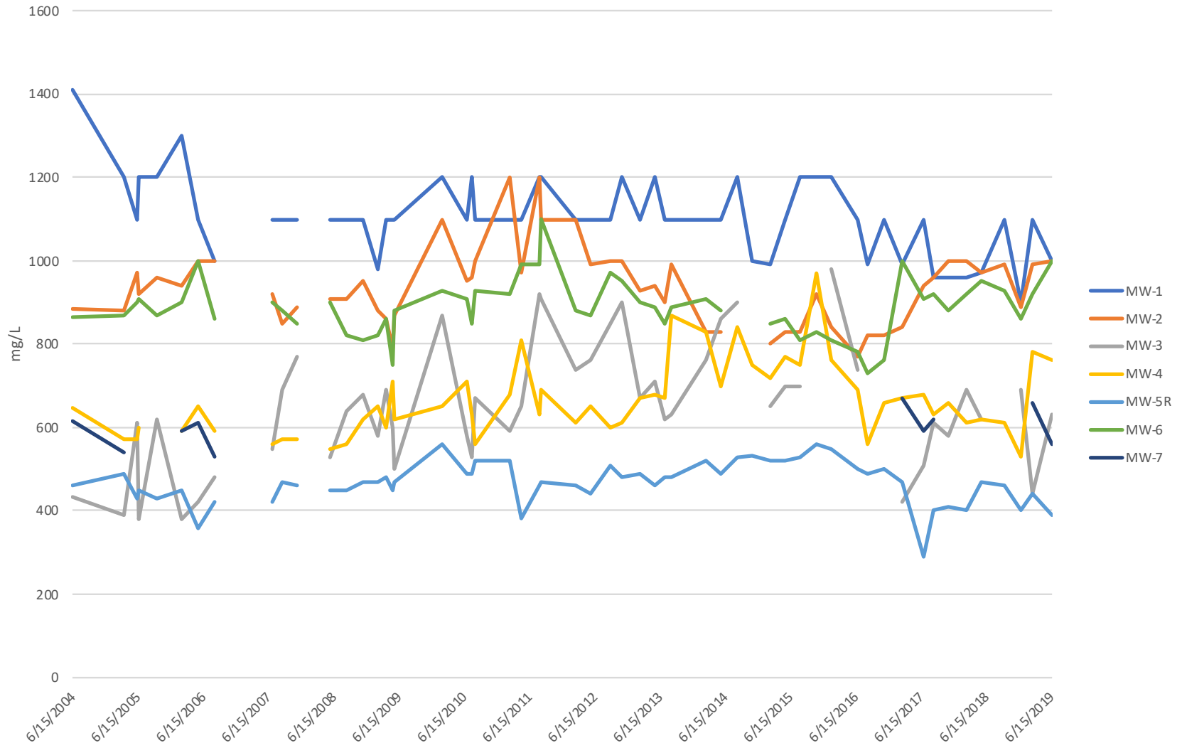
Chart 3 TDS Trends 2004-19
