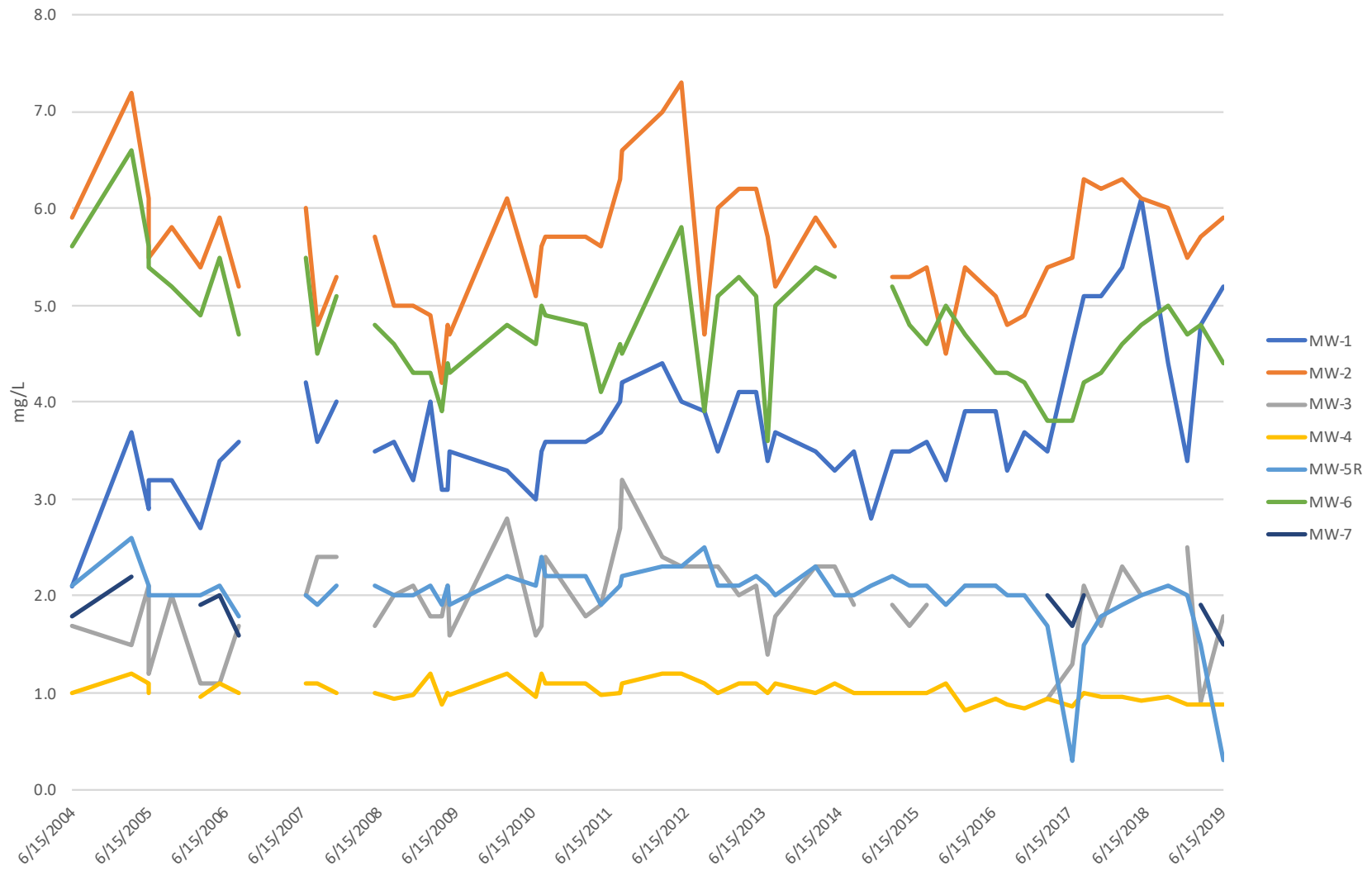
Chart 6 B Trends 2004-19
