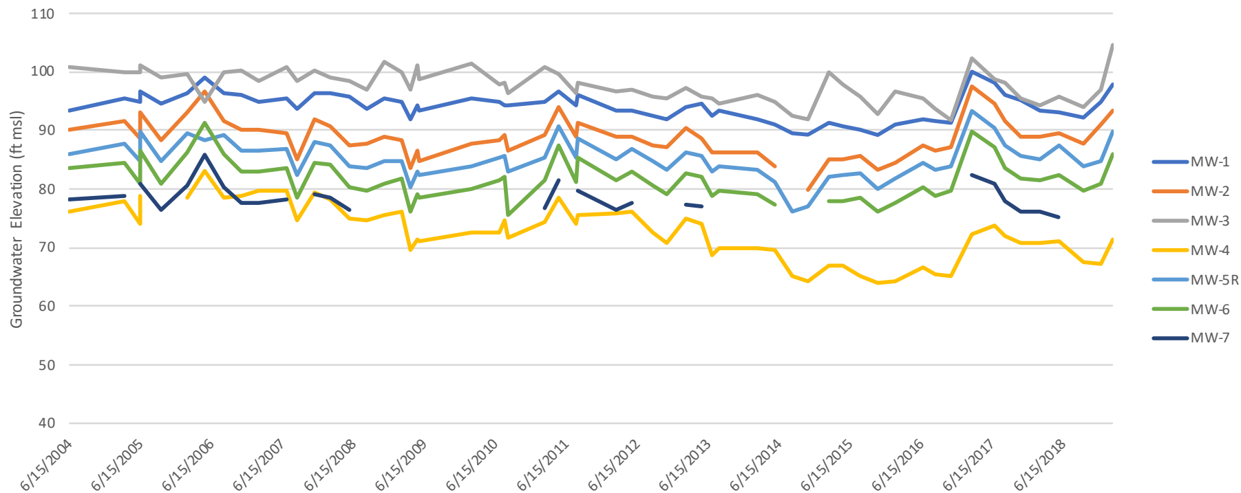
Chart 1 Water Levels 2004-19
