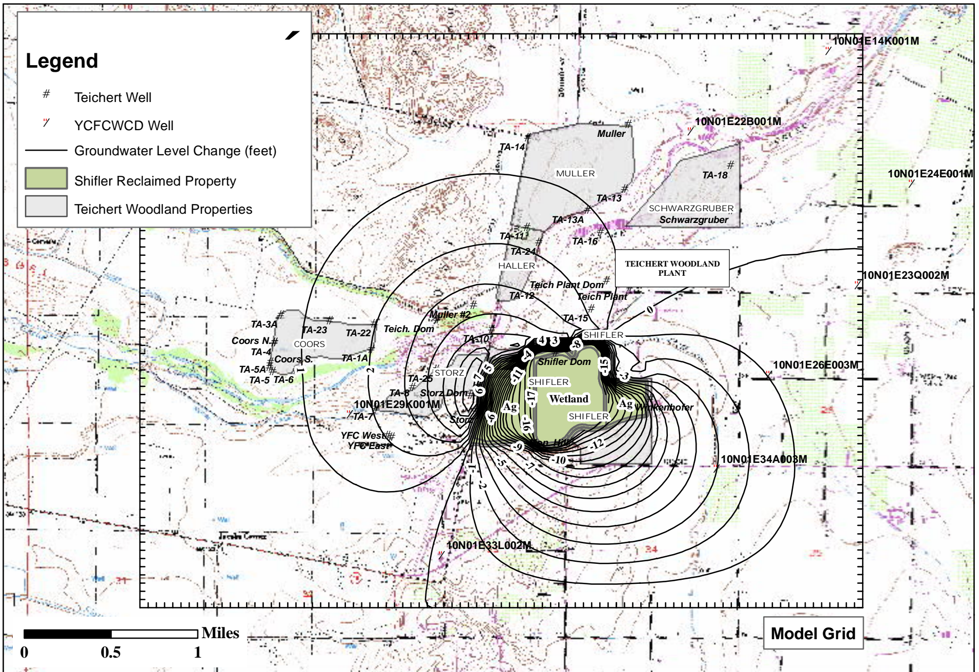
Figure 6a Simulated Contours, Equal Groundwater Level Change, Baseline vs Scenario 2A, Layer 1 Teichert Woodland Plant Area
