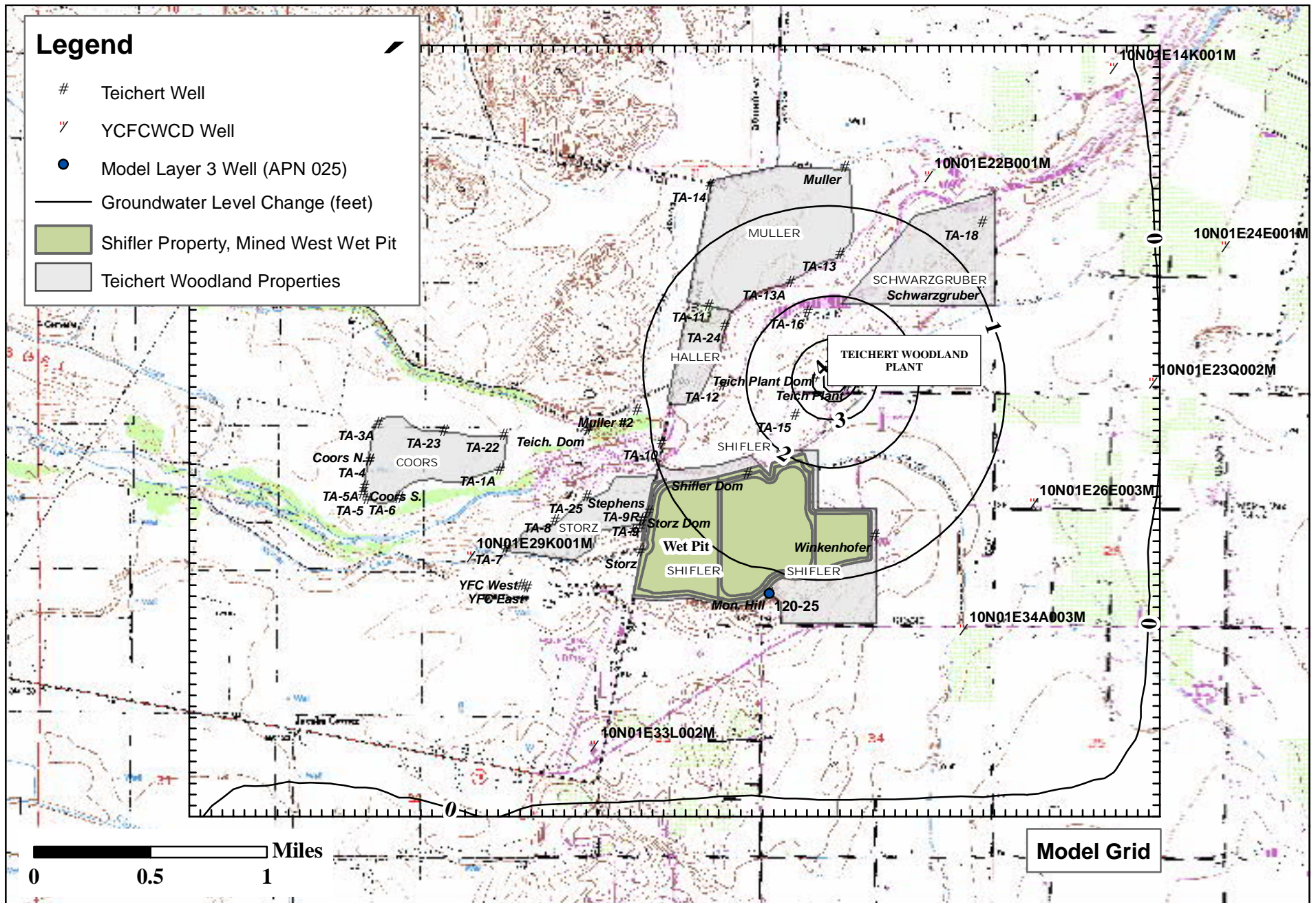
Figure 4c Simulated Contours, Equal Groundwater Level Change, Baseline vs Scenario 1A, Layer 3 Teichert Woodland Plant Area
