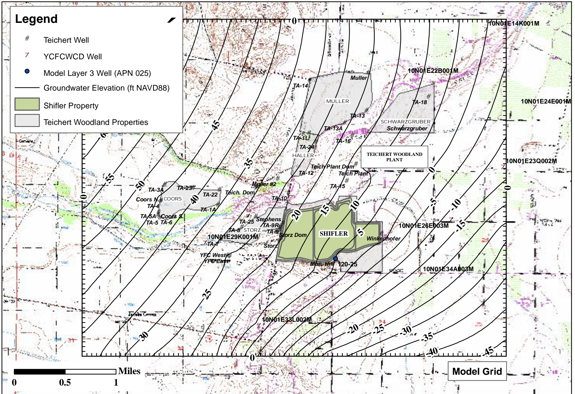
Figure 2c Simulated Contours of Equal Groundwater Elevation, Calibrated Baseline Model, Layer 3 Teichert Woodland Plant Area
