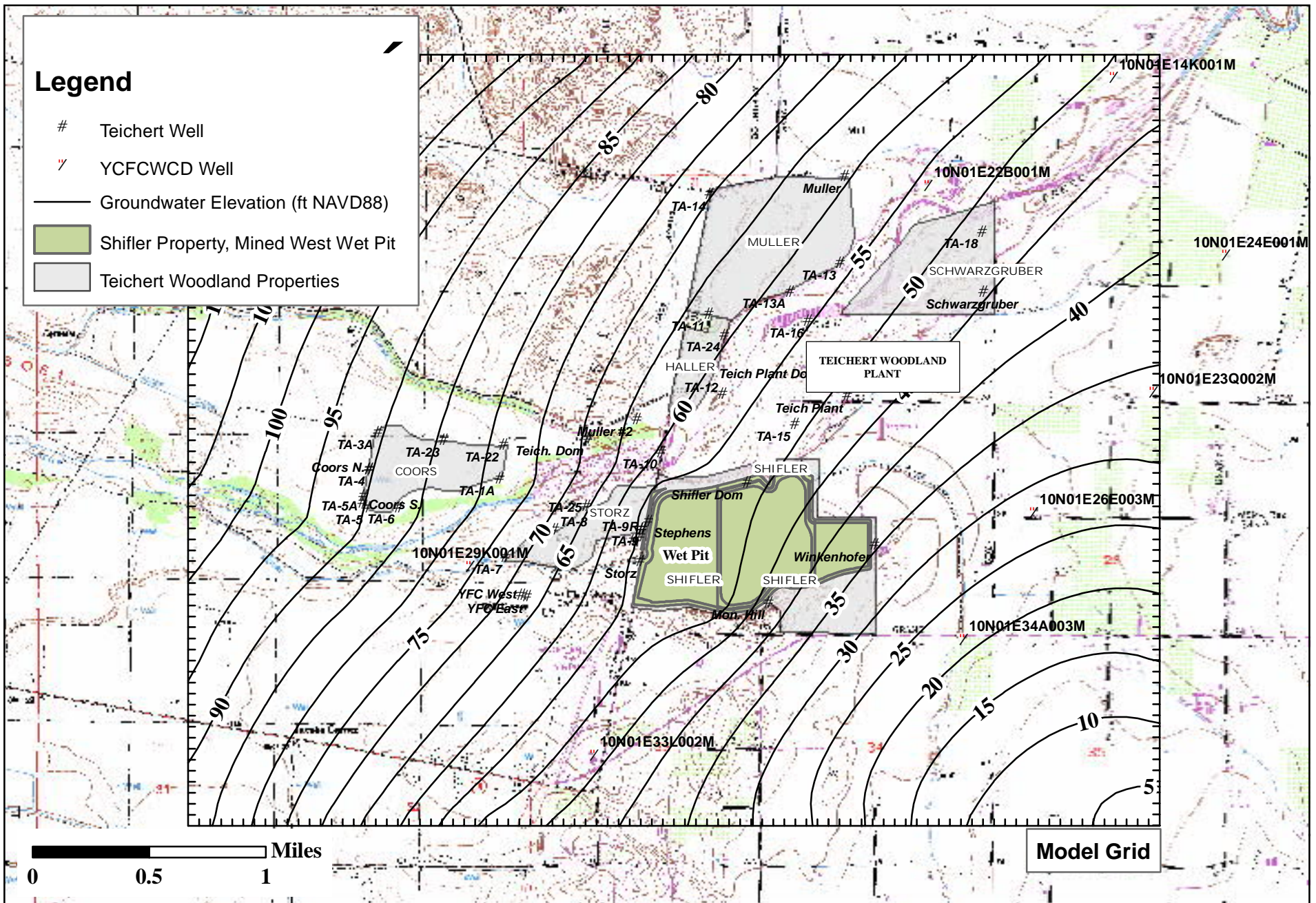
Figure 3a Simulated Contours of Equal Groundwater Elevation, Scenario 1A, Layer 1 Teichert Woodland Plant Area
