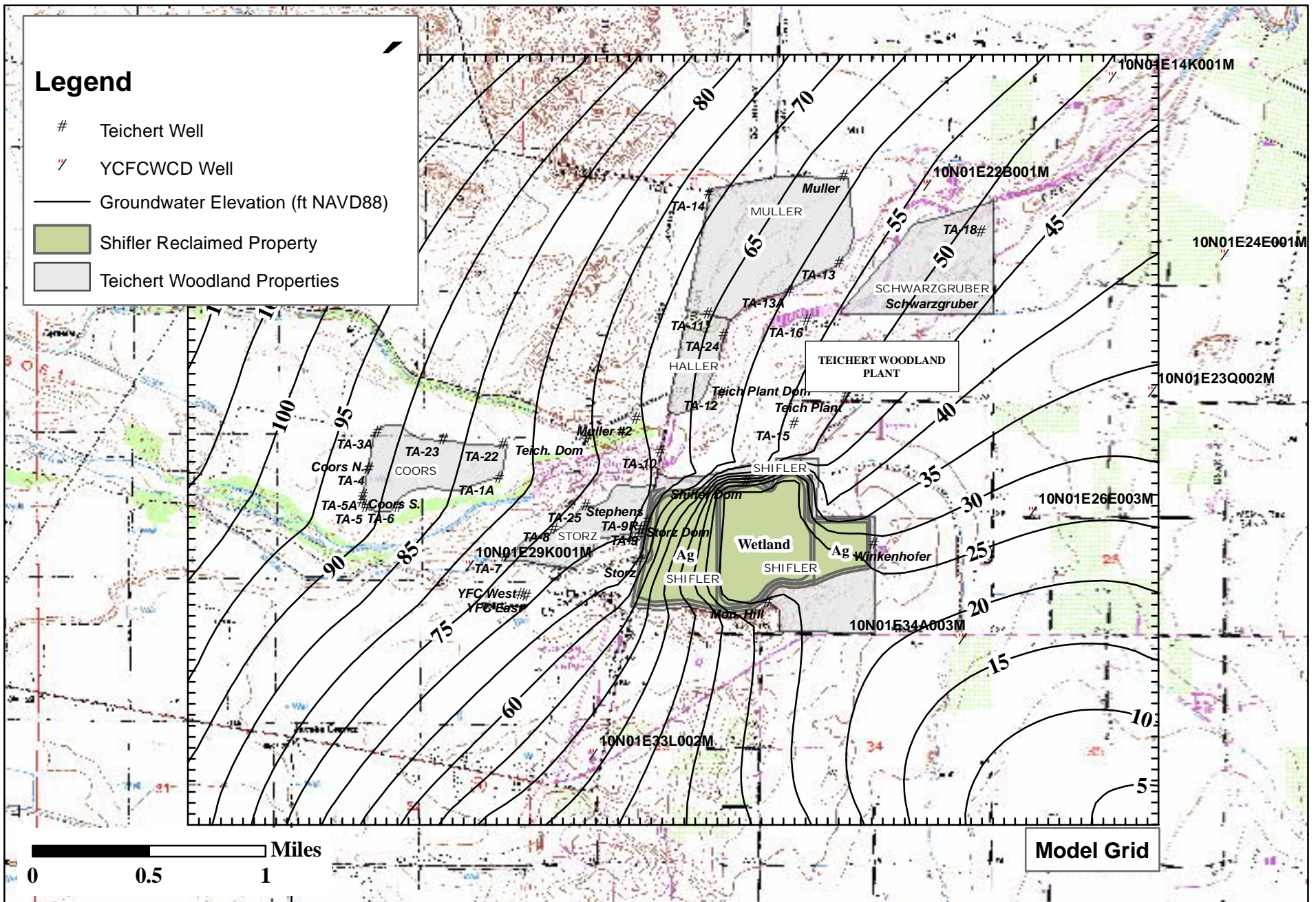
Figure 5a Simulated Contours of Equal Groundwater Elevation, Scenario 2A, Layer 1 Teichert Woodland Plant Area
