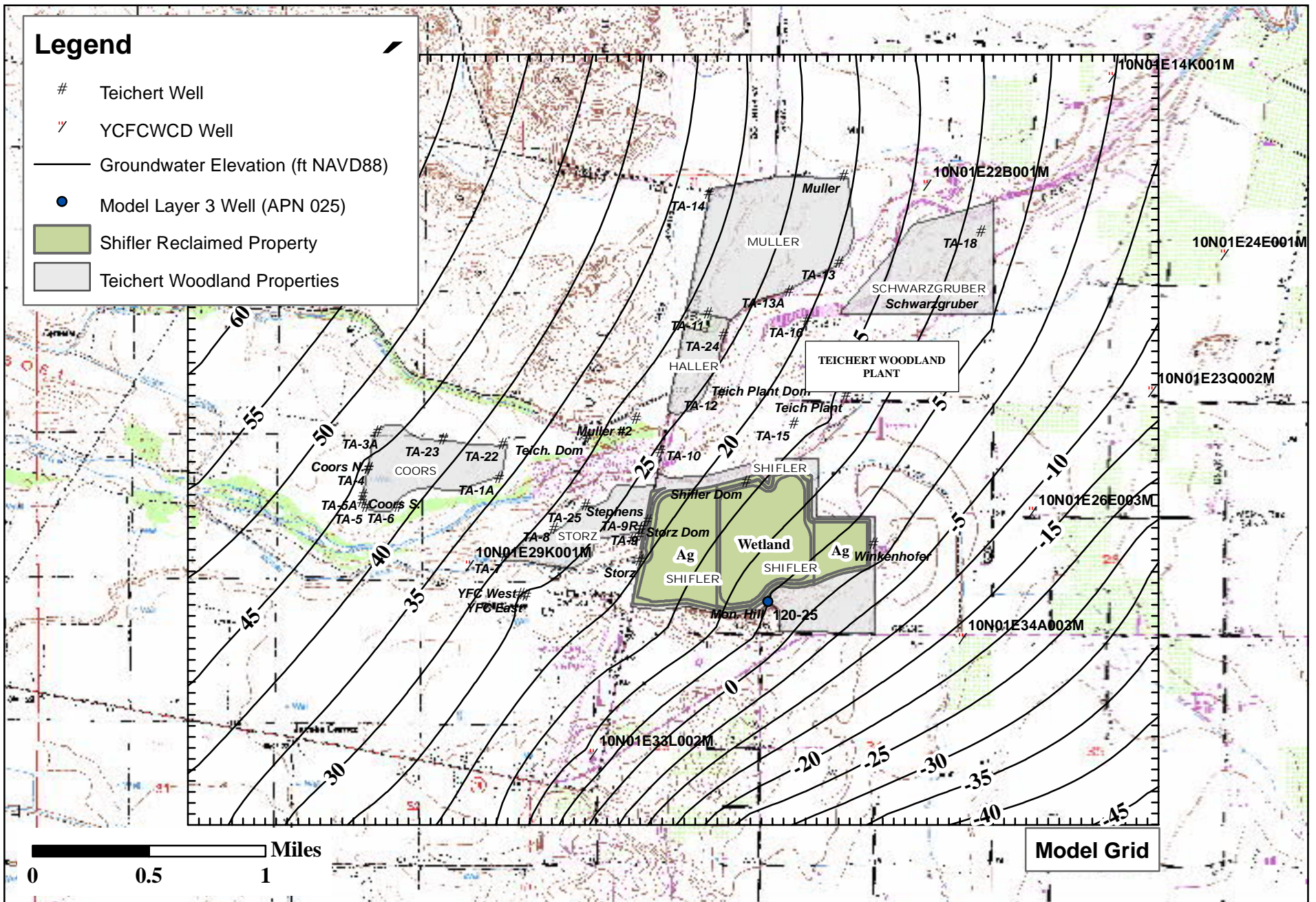
Figure 5c Simulated Contours of Equal Groundwater Elevation, Scenario 2A, Layer 3 Teichert Woodland Plant Area
