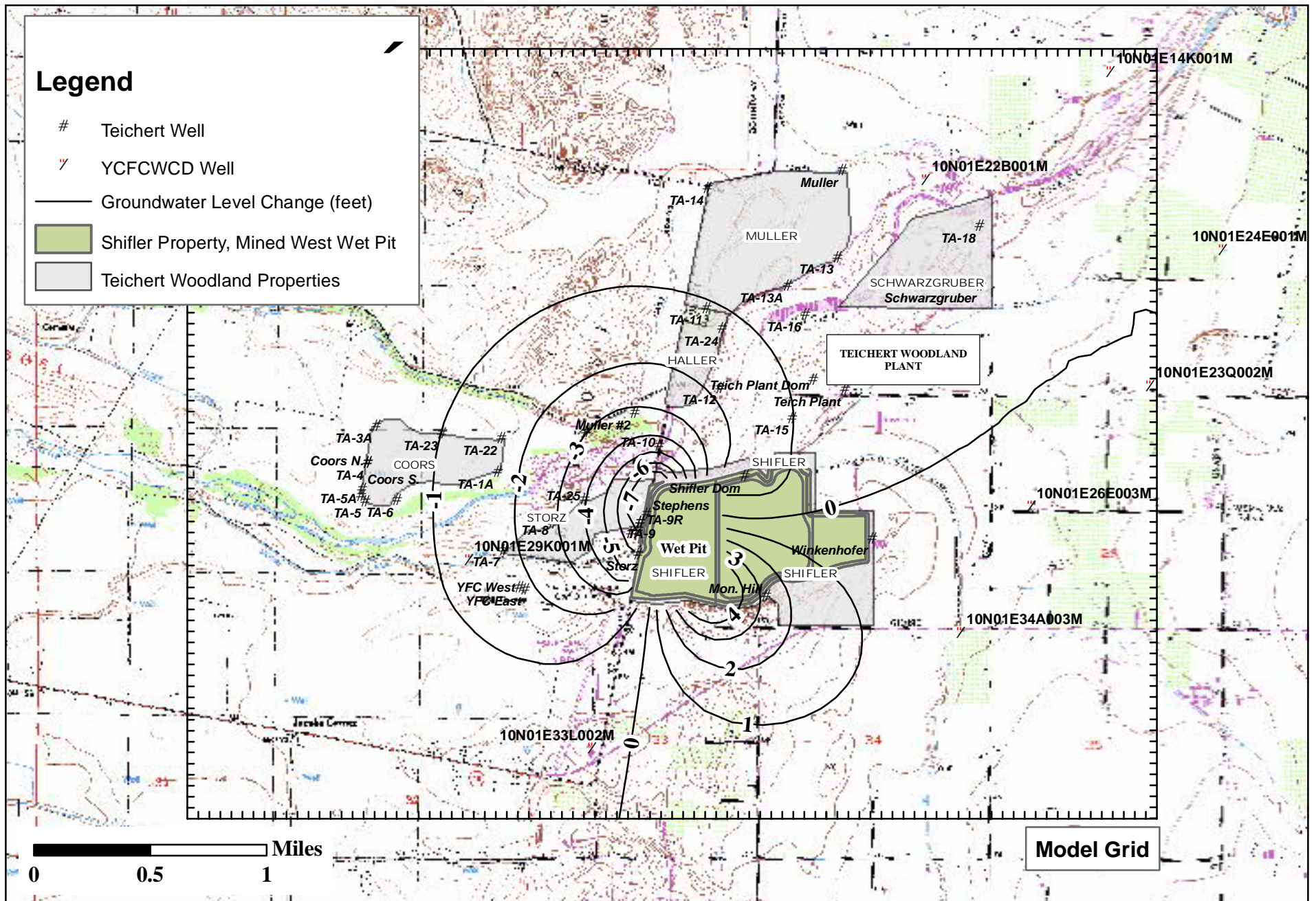
Figure 4a Simulated Contours, Equal Groundwater Level Change, Baseline vs Scenario 1A, Layer 1 Teichert Woodland Plant Area
