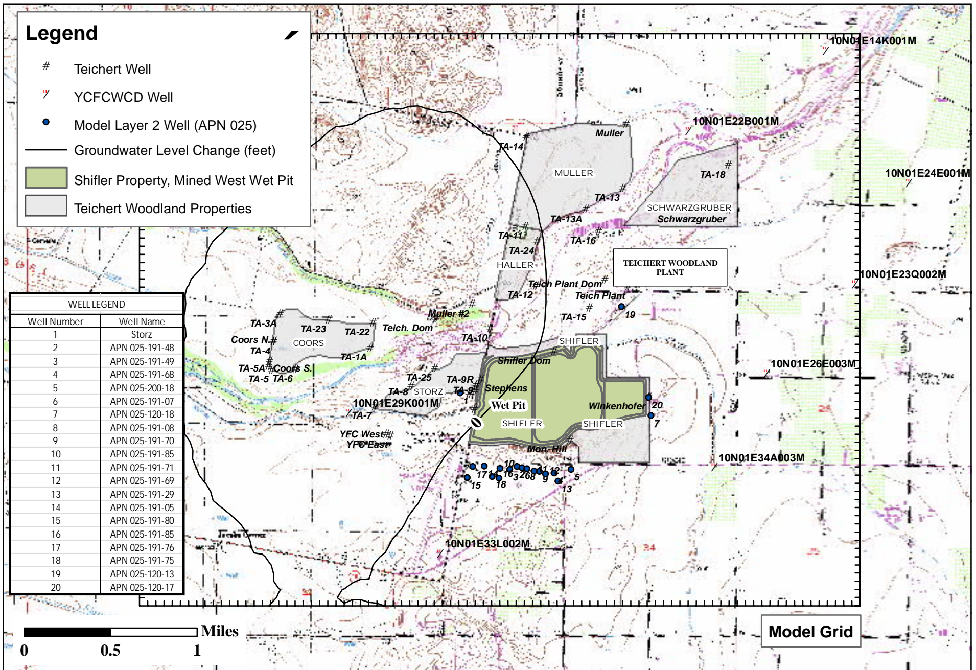
Figure 4b Simulated Contours, Equal Groundwater Level Change, Baseline vs Scenario 1A, Layer 2 Teichert Woodland Plant Area
