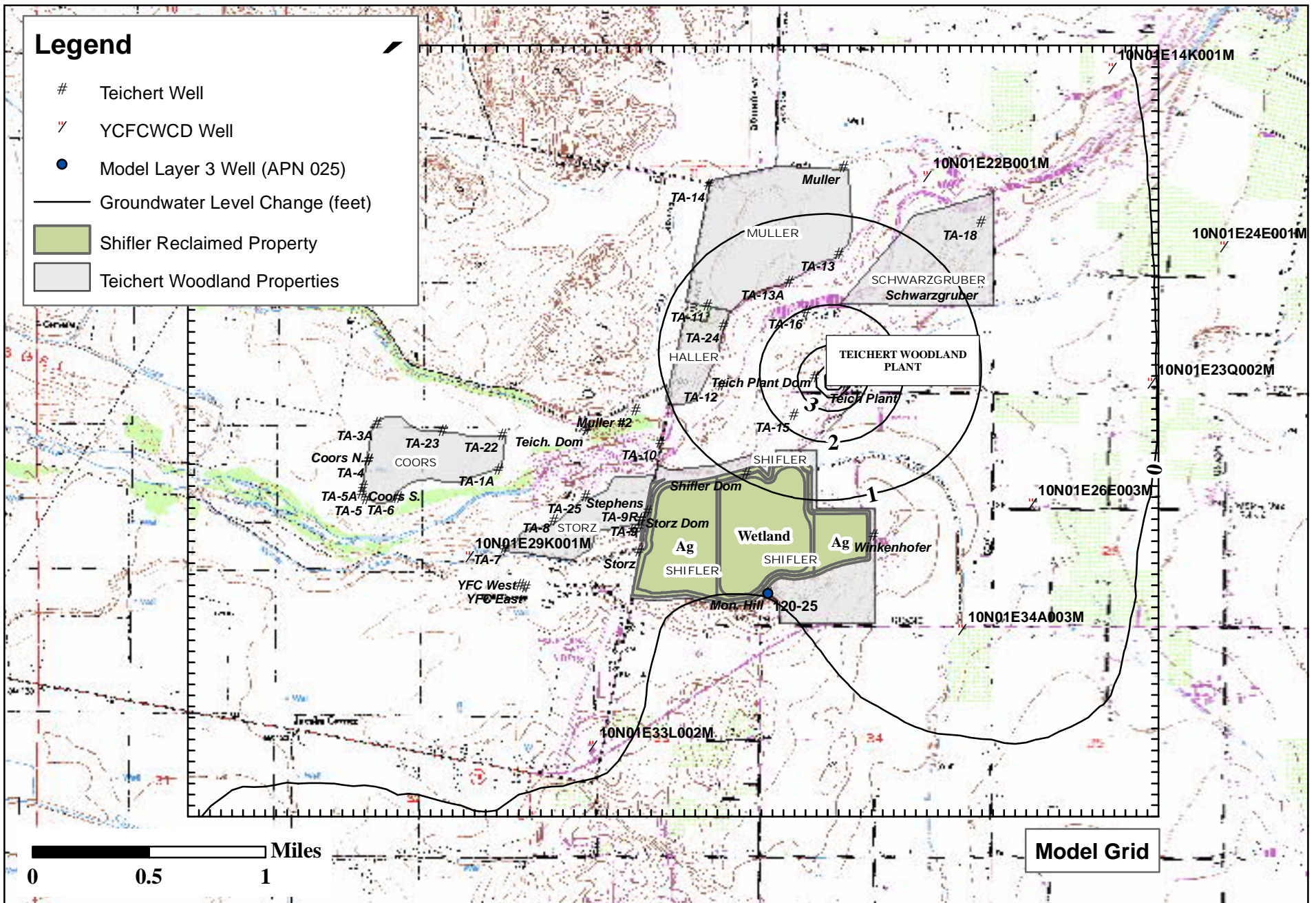
Figure 6c Simulated Contours, Equal Groundwater Level Change, Baseline vs Scenario 2A, Layer 3 Teichert Woodland Plant Area
