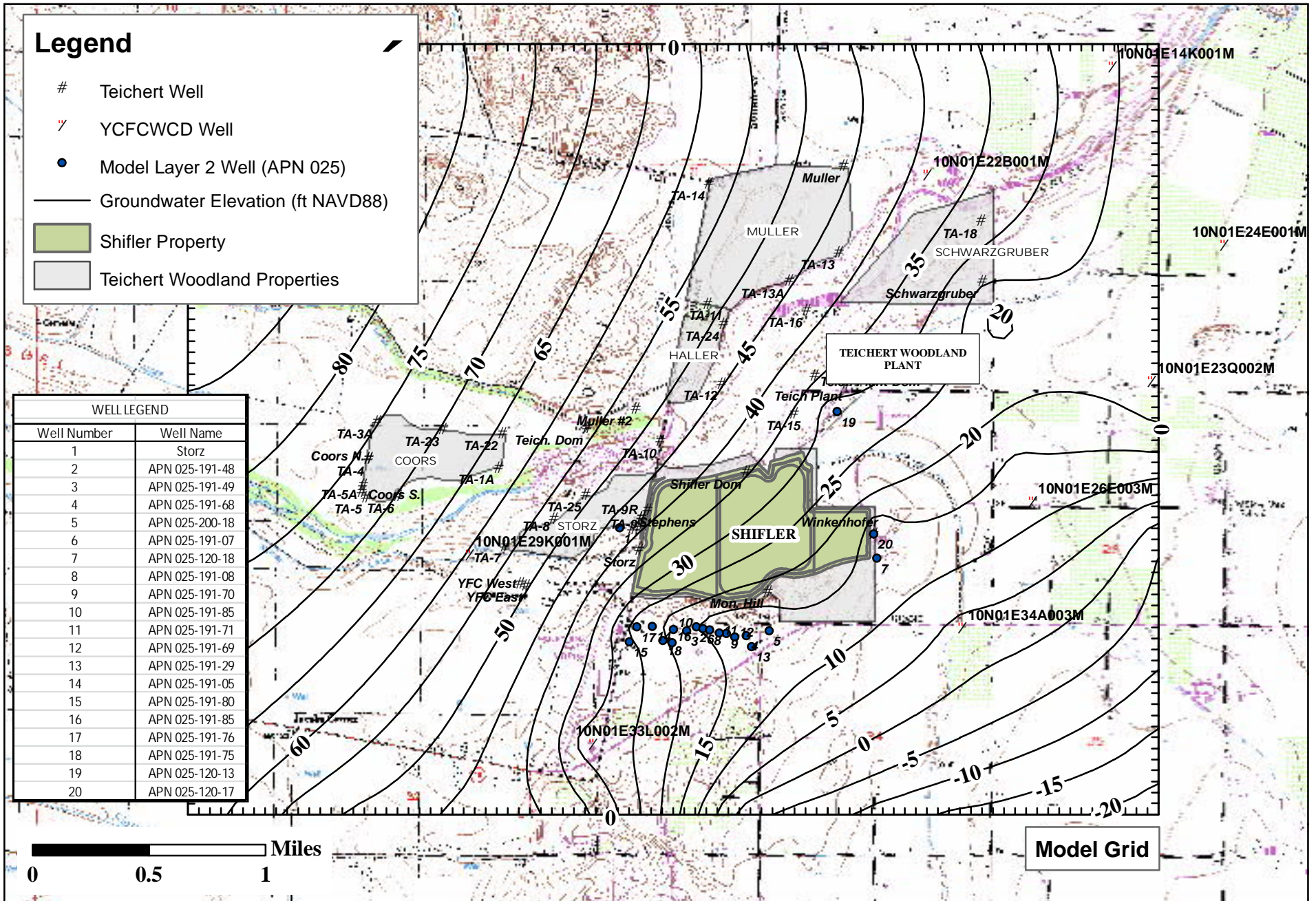
Figure 2b Simulated Contours of Equal Groundwater Elevation, Calibrated Baseline Model, Layer 2 Teichert Woodland Plant Area
