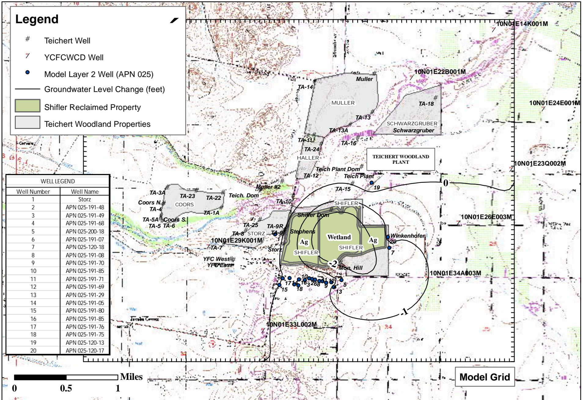
Figure 6b Simulated Contours, Equal Groundwater Level Change, Baseline vs Scenario 2A, Layer 2 Teichert Woodland Plant Area
