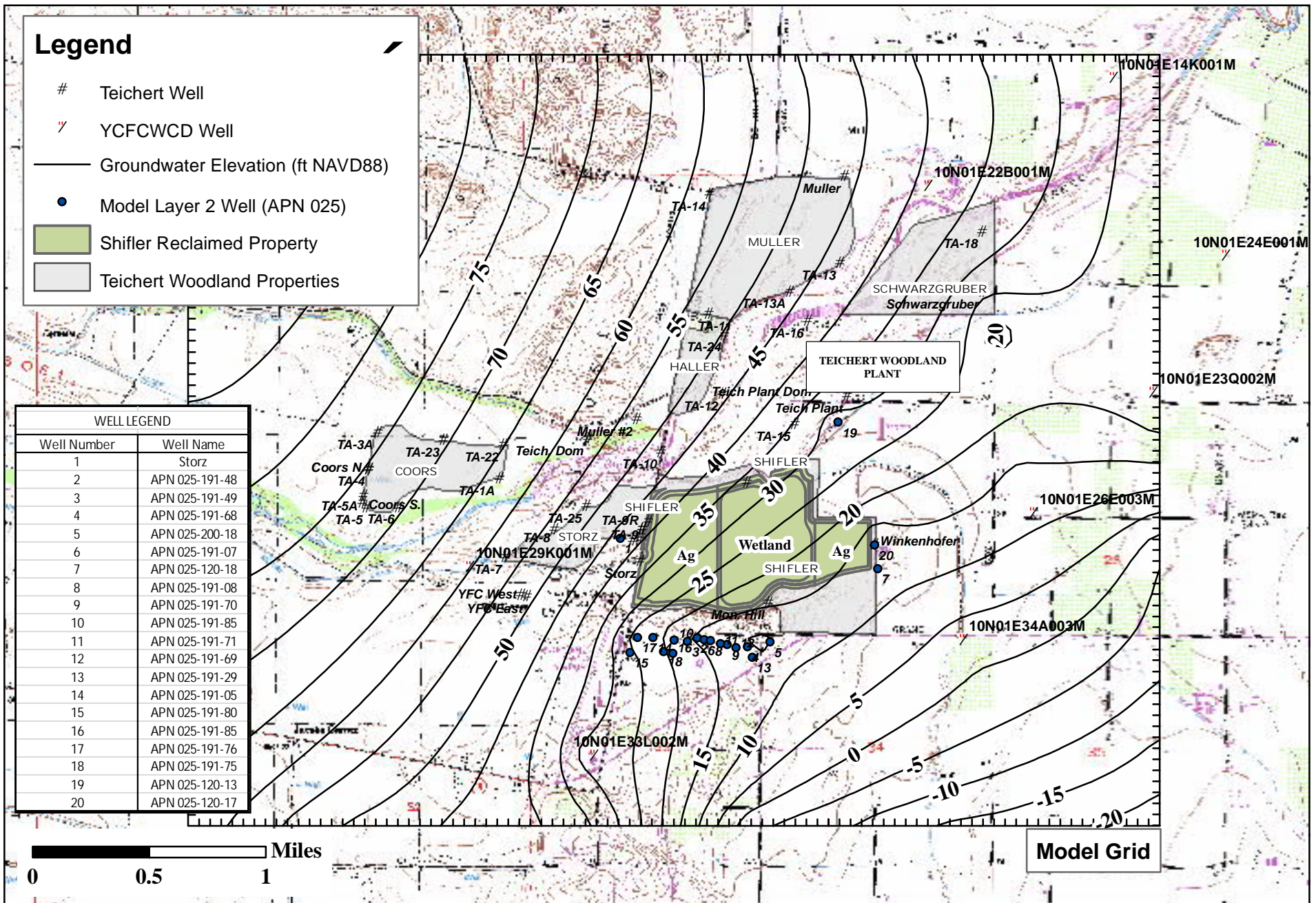
Figure 5b Simulated Contours of Equal Groundwater Elevation, Scenario 2A, Layer 2 Teichert Woodland Plant Area
