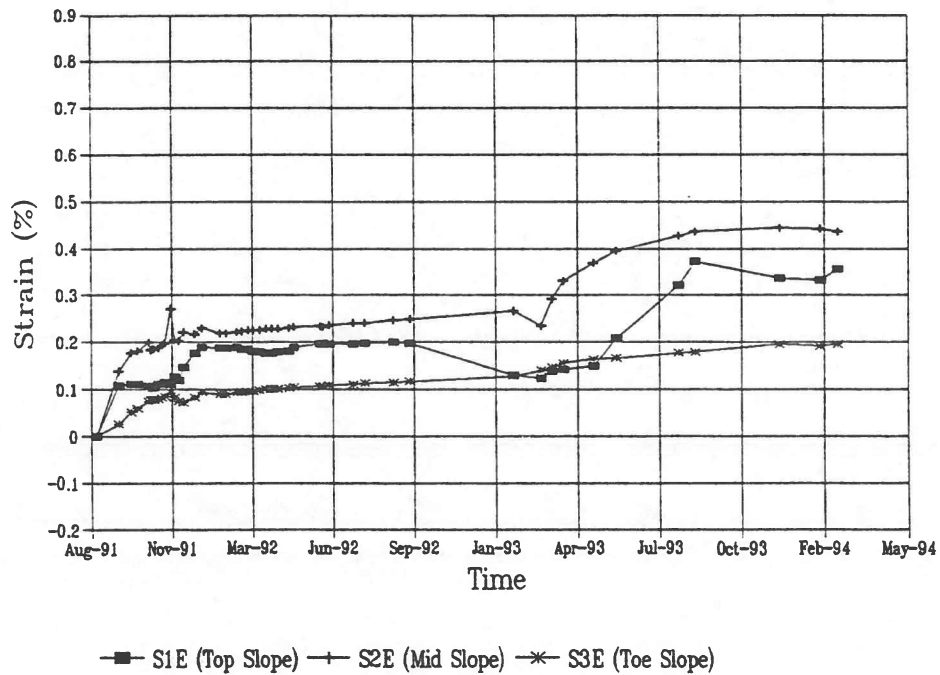
Figure 12. Strain Responses of Station E Gauges.
