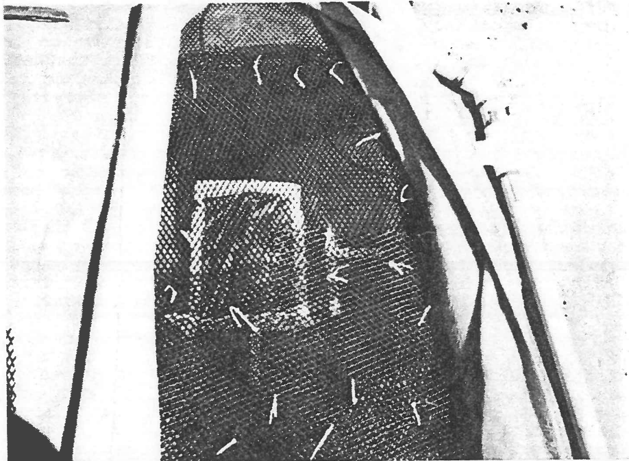
Figure 6. Installed Strain Gauges (Below Geonet) with PVC Conduit for Leadwires Above the Composite Liner.
