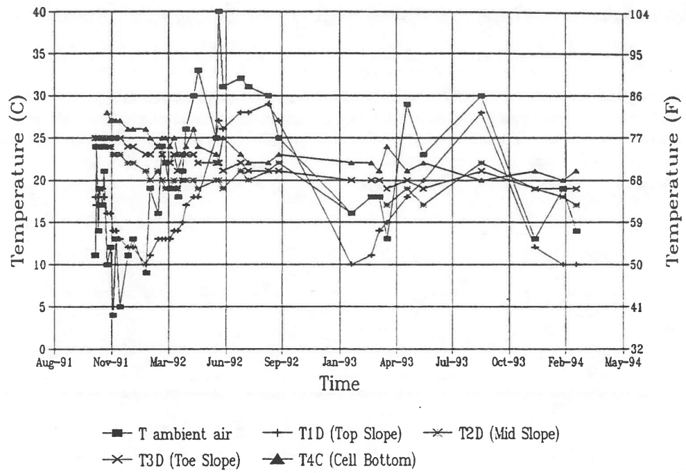
Figure 7. Temperature Responses of Station C and Station D Thermocouples.
